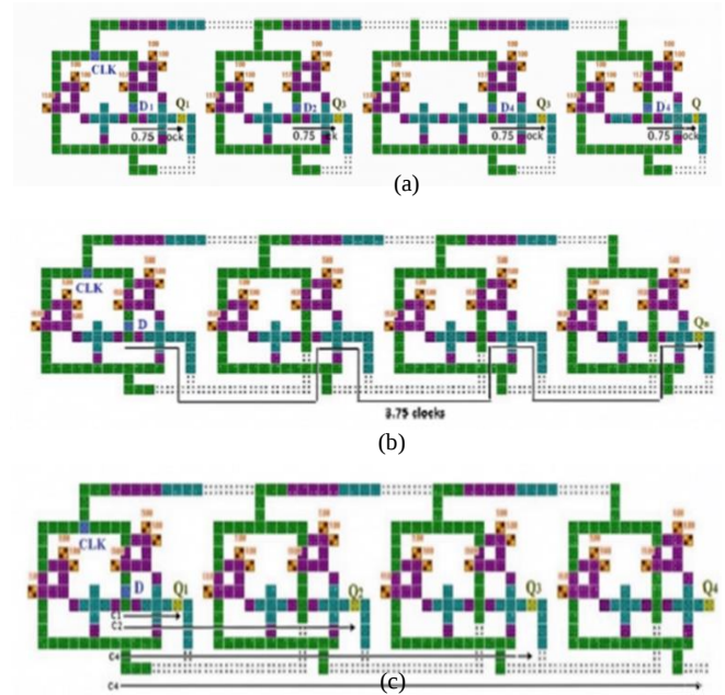
Fig. 6. The physical structure of the shift registers presented in [10] a) PIPO b) SISO c) SIPO.
