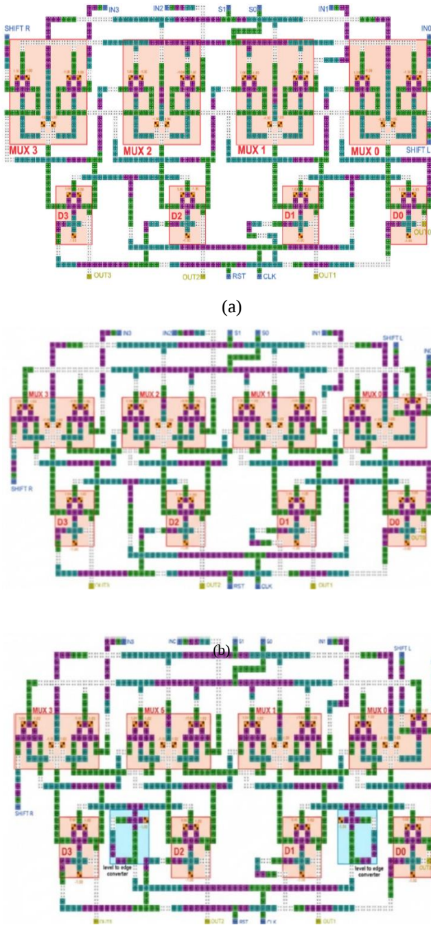
Fig. 7. The physical structure of the shift registers presented in [8] a) using D-latches with reset ability b) the improved model and c) the proposed model with rising edge clock. (c)
