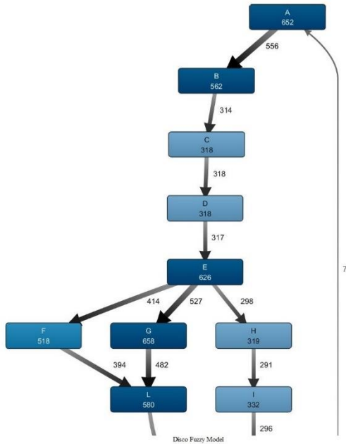
Fig. 4. Discovered models based on the fuzzy method
